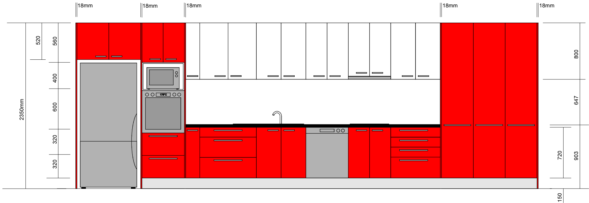
2350mm High Kitchen (gas cooktop)
